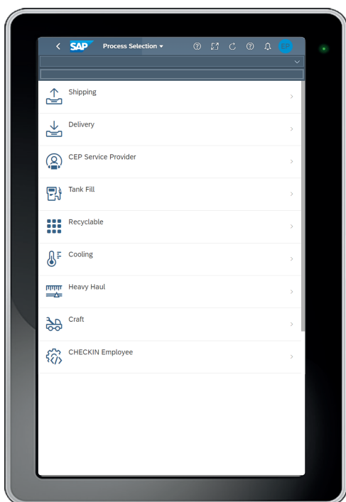
FlexYard App „Process Selection“
